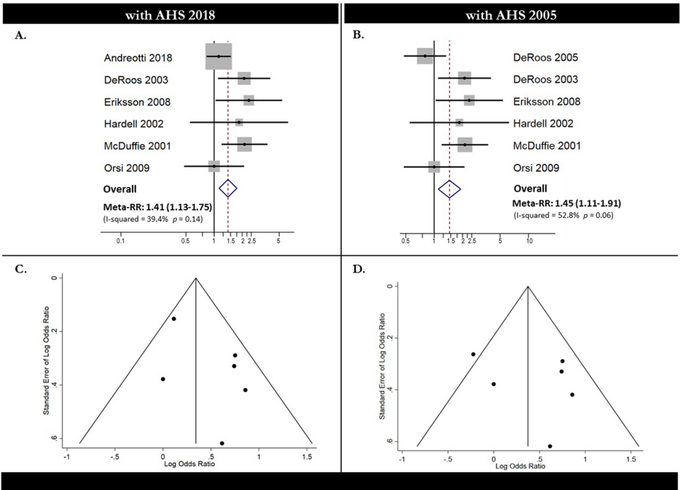
Fig. 3. Findings from major meta-analyses. 3A-B: Forest plots for meta-analyses using AHS 2018 (3A) and AHS 2005 (3B); 3C-D: Funnel plots for meta-analyses using AHS 2018 (3C) and AHS 2005 (3D).
